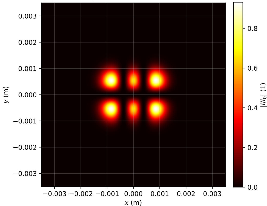
Intensity profile I(x, y, z = 0.796)/I_0 , P_{in}=0.5P_{cr} , artificial time
